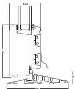
Low aluminium threshold, inward opening doors
